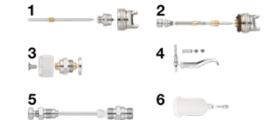
CAR G04HVLP paint spray gun parts
