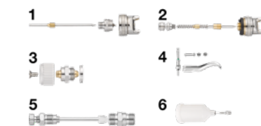
CAR G04 paint spray gun parts
