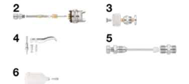
G04HWW water-based paint spray gun parts
